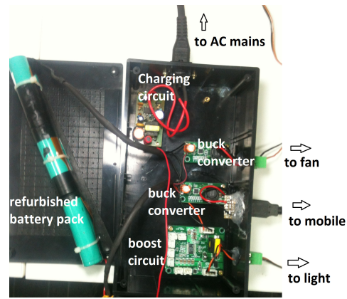
Figure 1: Component details of an UrJar prototype built using discarded laptop batteries.
