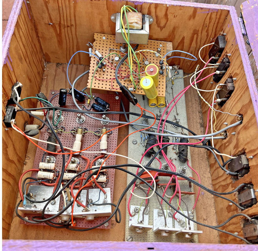
Figure 2-1: A stereo, 3-band Color Organ circuit built by my advisor in 1972.
