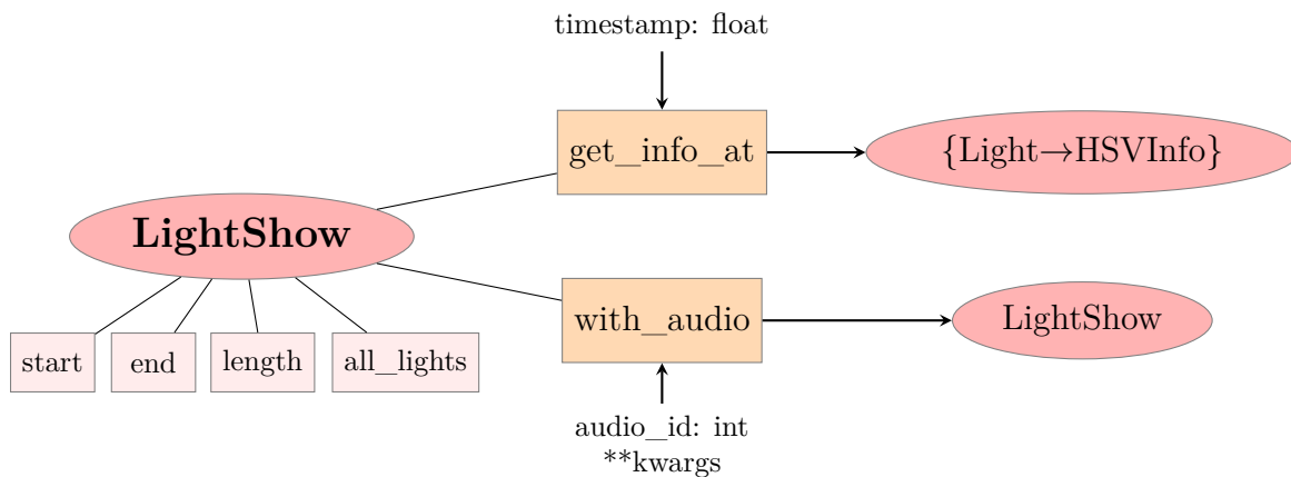
Figure 4-2: The LightShow Interface
