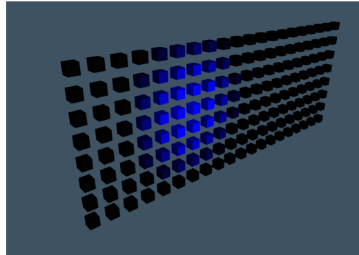
After using on_shape to project a constant blue LightShow onto this panel using the sphere, this is the result.
