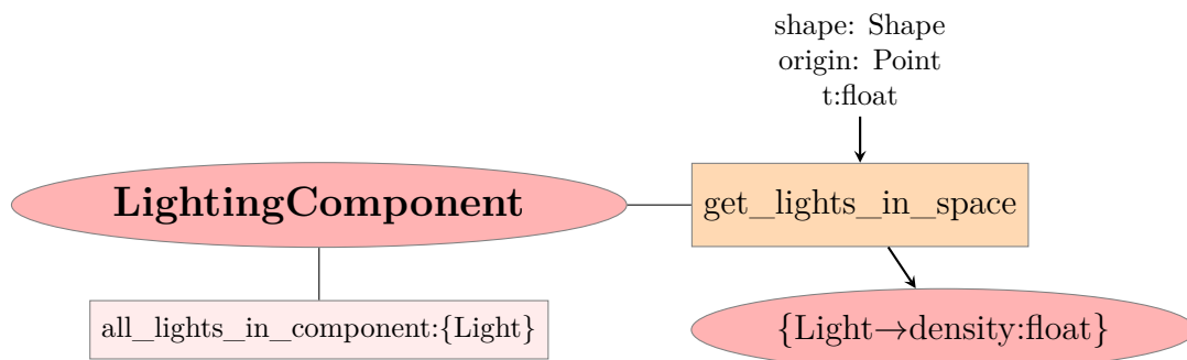
Figure 4-4: The LightingComponent Interface
