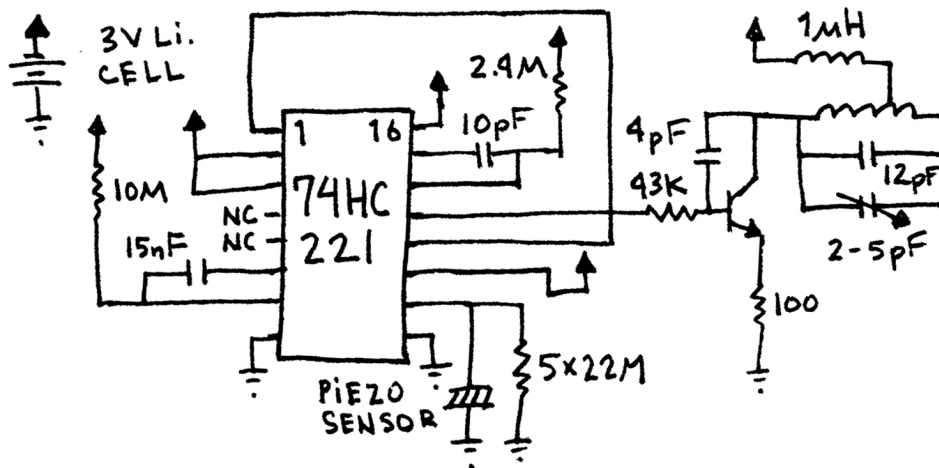
Figure 3.1.7: Schematic of Revision Five Sensor
