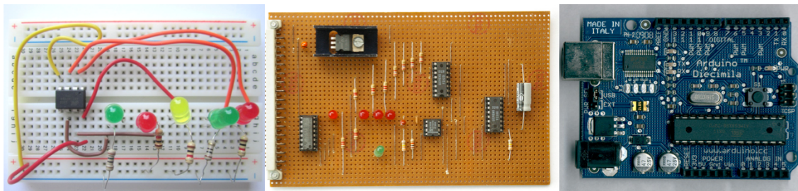
Figure 2.3. From left to right: breadboard circuit, protoboard circuit (image by smial) and printed circuit board (image by Remko van Dokkum).
