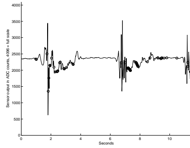
(c) Accelerometer 3
