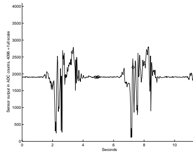
(e) Gyro 2
