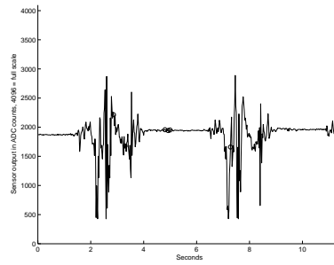
(c) Accelerometer 3
