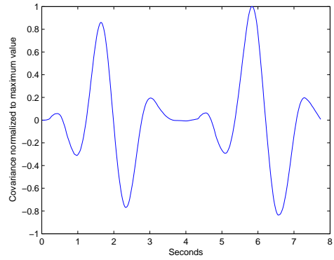
(b) Wave: covariance of node 1 with node 3
