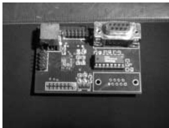
Figure A-6: Communications board populated
