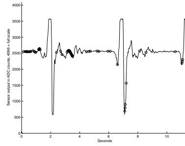
(b) Accelerometer 2
