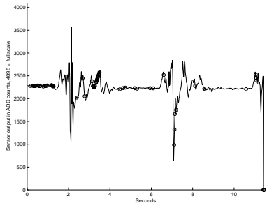
(a) Accelerometer 1
