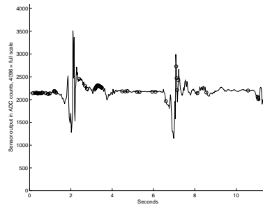
(c) Accelerometer 3
