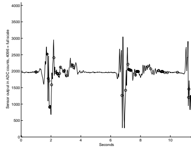
(e) Gyro 2
