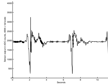
(e) Gyro 2
