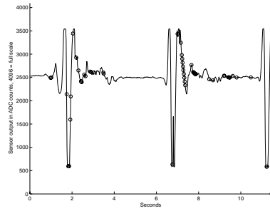
(b) Accelerometer 2
