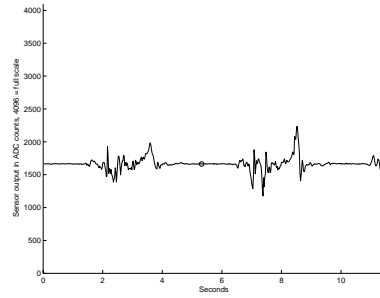
(e) Gyro 2
