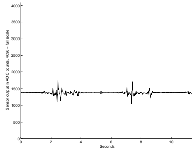
(b) Accelerometer 2
