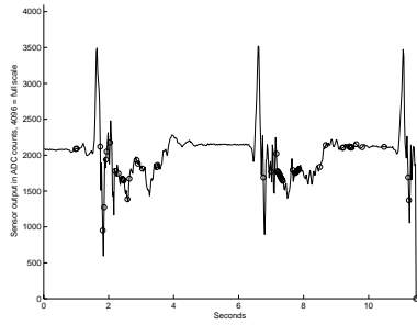
(a) Accelerometer 1
