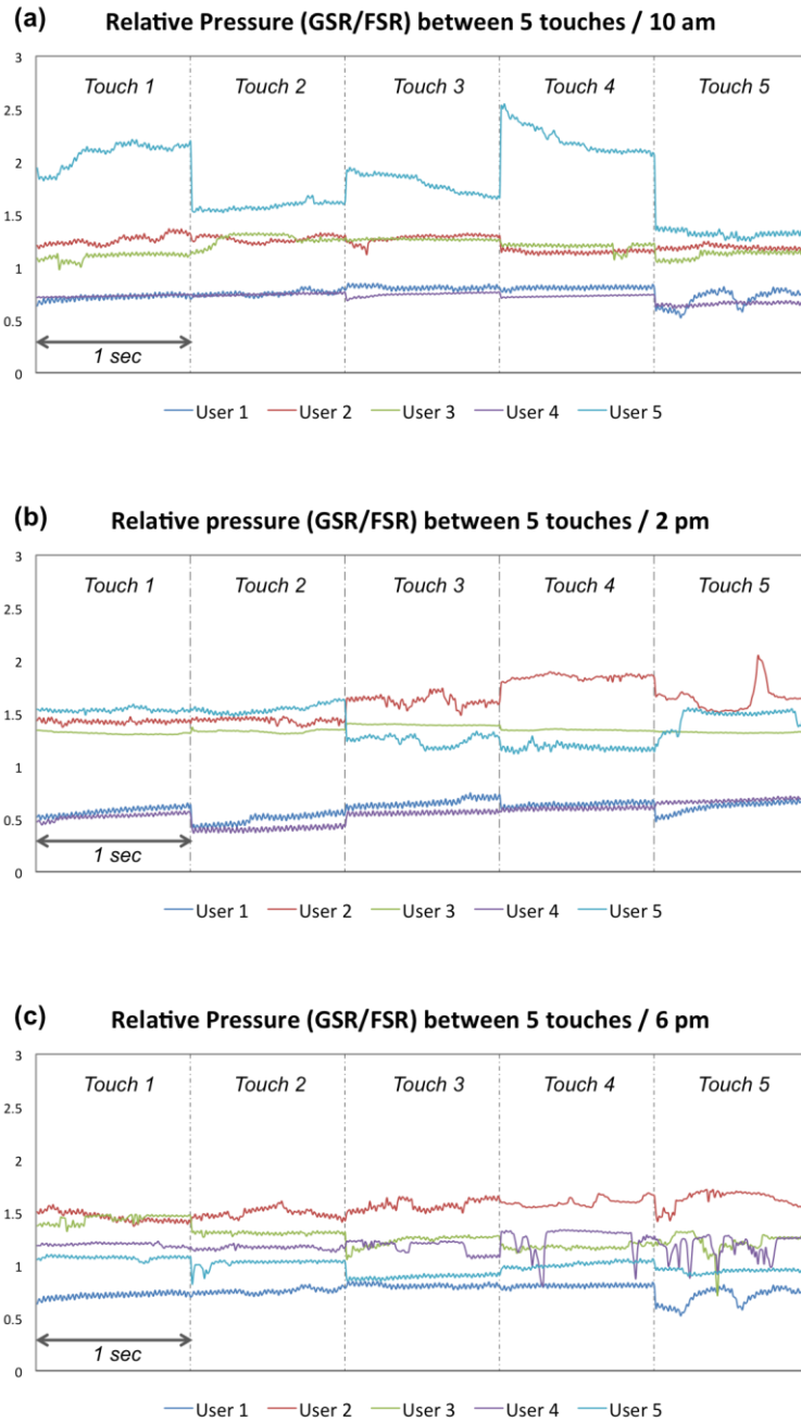
Figure 7.11 Relative Pressure between 5 touch inputs among 5 users across time. Each inconiguous input is 1000 samples with duration of 1 second.
