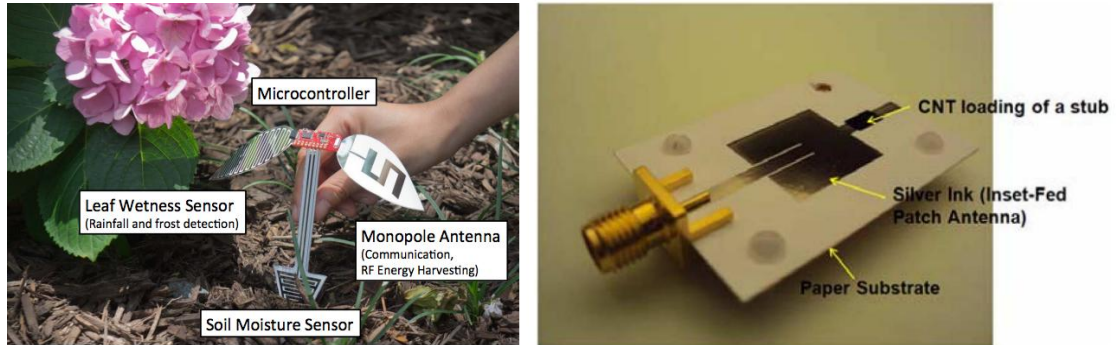
Figure 2.9 Left: SenSprout: inkjet-printed soil moisture and leaf wetness sensor. Right: RFID tag module designed on flexible substrate, with inkjet-printed single wall carbon nanotubes (SWCNT) film as a load.
