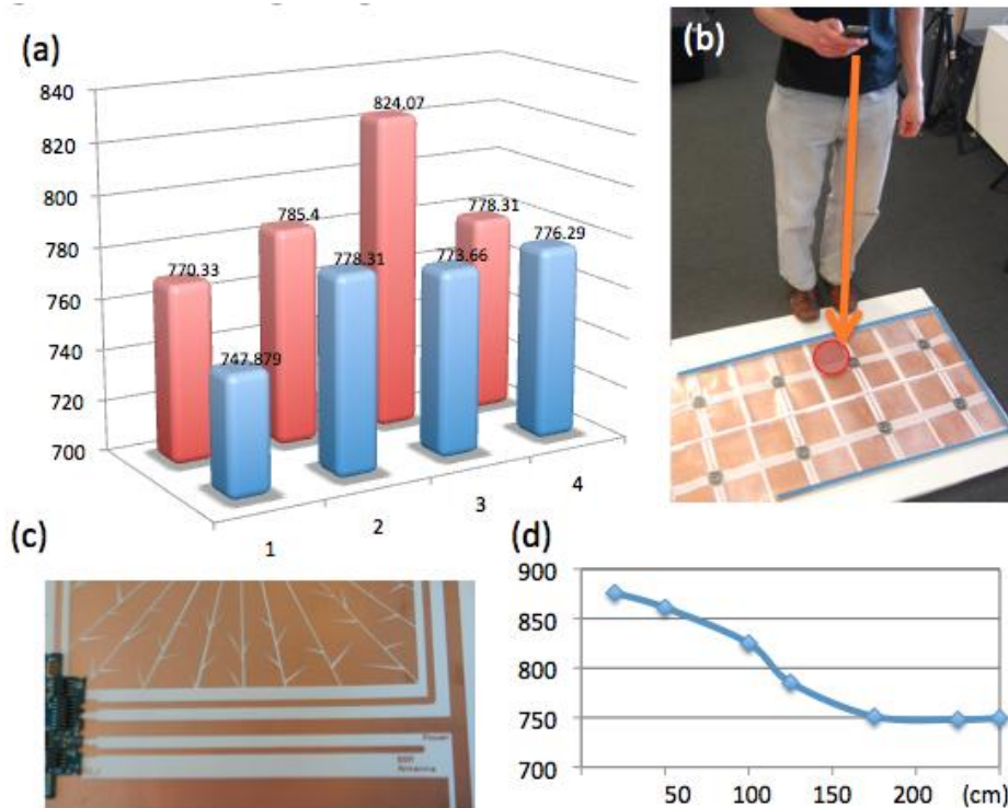
Figure 6.14. (a) Signal response versus sensing unit location when a GSM device is held 1m from the surface. (b) Illustration of the experimental setup. (c) Close up of the tile GSM antenna. (d) GSM signal strength versus distance.
