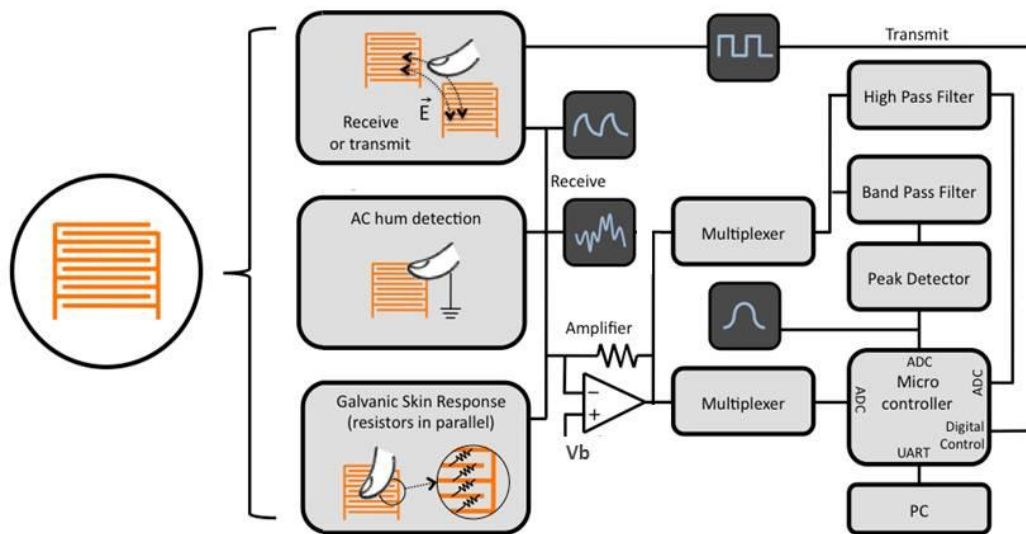
Figure 7.6. PrintSense hardware.
