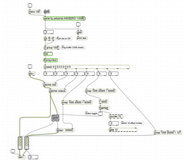
Figure 4.12. Example Max Patch for the Zebra Skin Interface.
