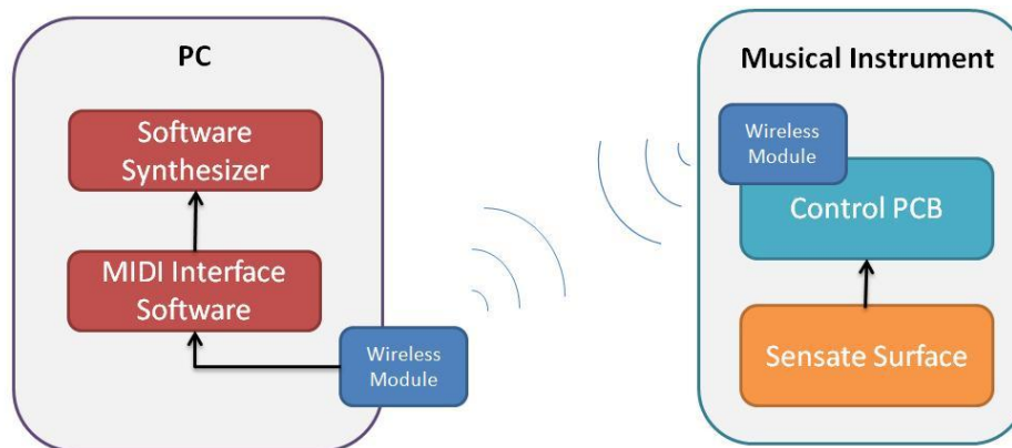
Figure 4.6. System block diagram – The main hardware is attached to a musical instrument or essentially any object. A sensate surface communicates with the control circuitry, which talks to a wireless module. The other end of the wireless data transmission sits on top of a computer, which parses and passes the information to MIDI interfacing software. The software then sends MIDI messages to a software synthesizer.
