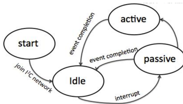
Figure 6.4. Basic operation of each slave sensor unit. Once an unit joins the I 2 c network, it enters a low-power idle mode and can be interrupted by piezo pickup, RF signals, or the network (signal detected from adjacent units) and enters presence sensing, interaction and recognition mode.
