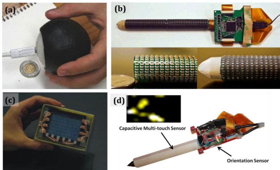
Figure 2.5 (a)The Tango: a tangible receptive whole-hand interface [36]. (b) FlexAura, a flexible near-surface range sensor [27], (c) The Bar of Soap, handheld devices that combine grasp and orientation sensing, (d) Grips and Multi-touch Pen [35].
