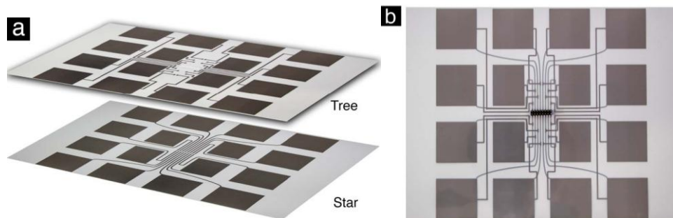
Figure 5.4: a) Prototype of a dual-layer sensor (b) with overlaid tree and star topologies (a) for a 4x4 sensor sheet. The tree topology is printed on a transparent PET film. Both layers are connected using 3M conductive z-Tape.
