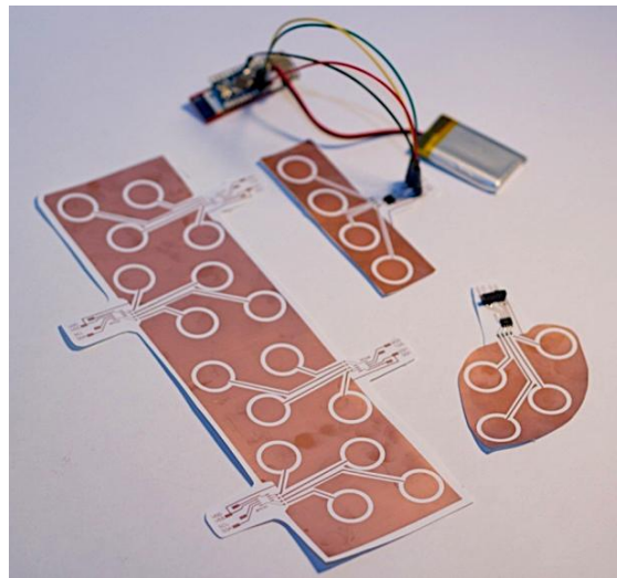
Figure 4.15. Toolkit for basic implementation. Two design patterns were made. Each battery-powered unit, as seen in the back, can transmit sensor data wirelessly though Bluetooth.
