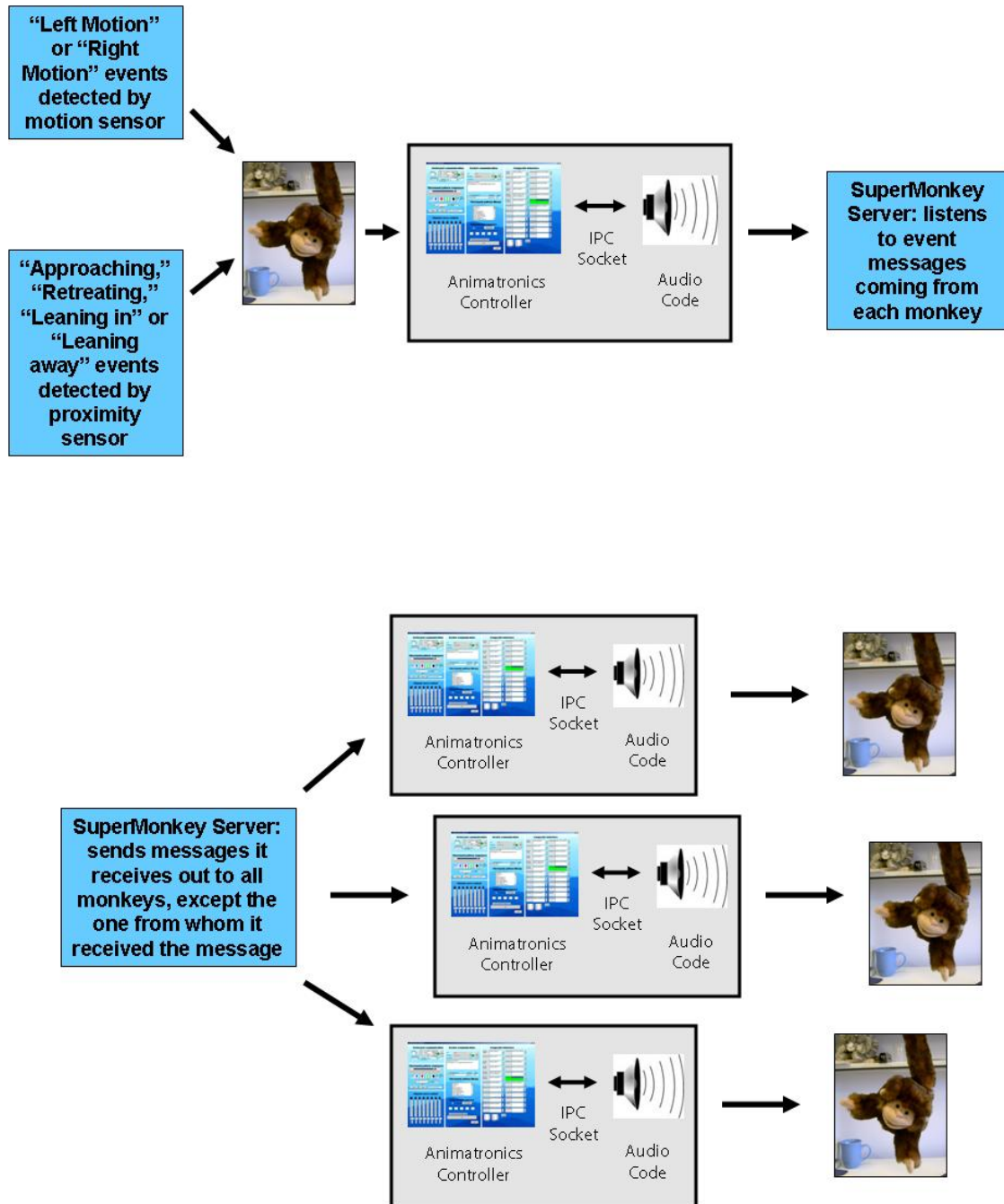
Figure 3-13. Flow of sensor event information from each monkey to the SuperMonkey Server, and then from the SuperMonkey Server back out to each monkey.
