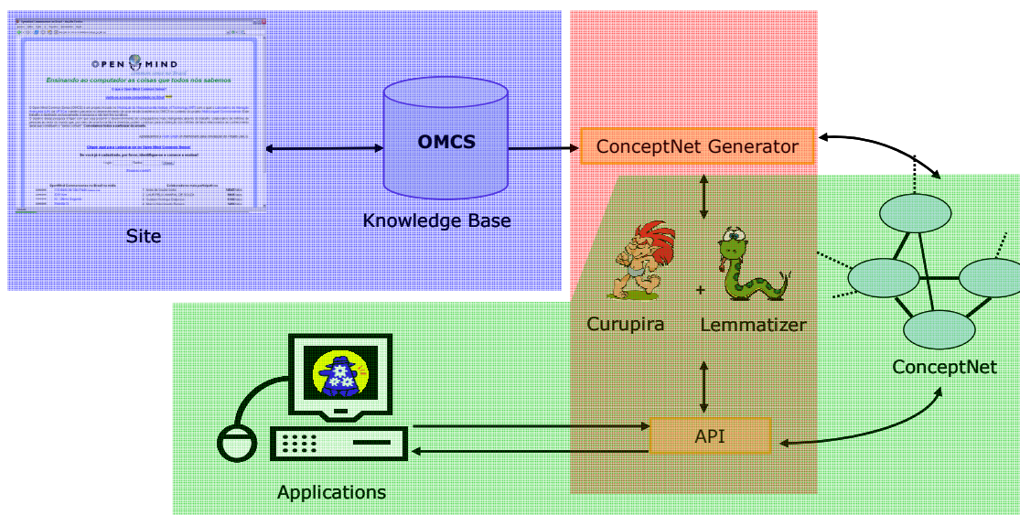
Figure 1. Open Mind Commonsense Project Architecture
