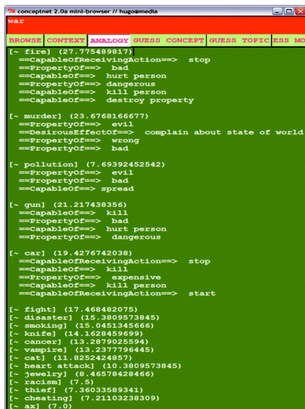
Fig 4 The results of a GetAnalogousConcepts() query for 'war' are displayed in the ConceptNet knowledge browser. Structures shared in the analogy are only shown for the first five concepts.
